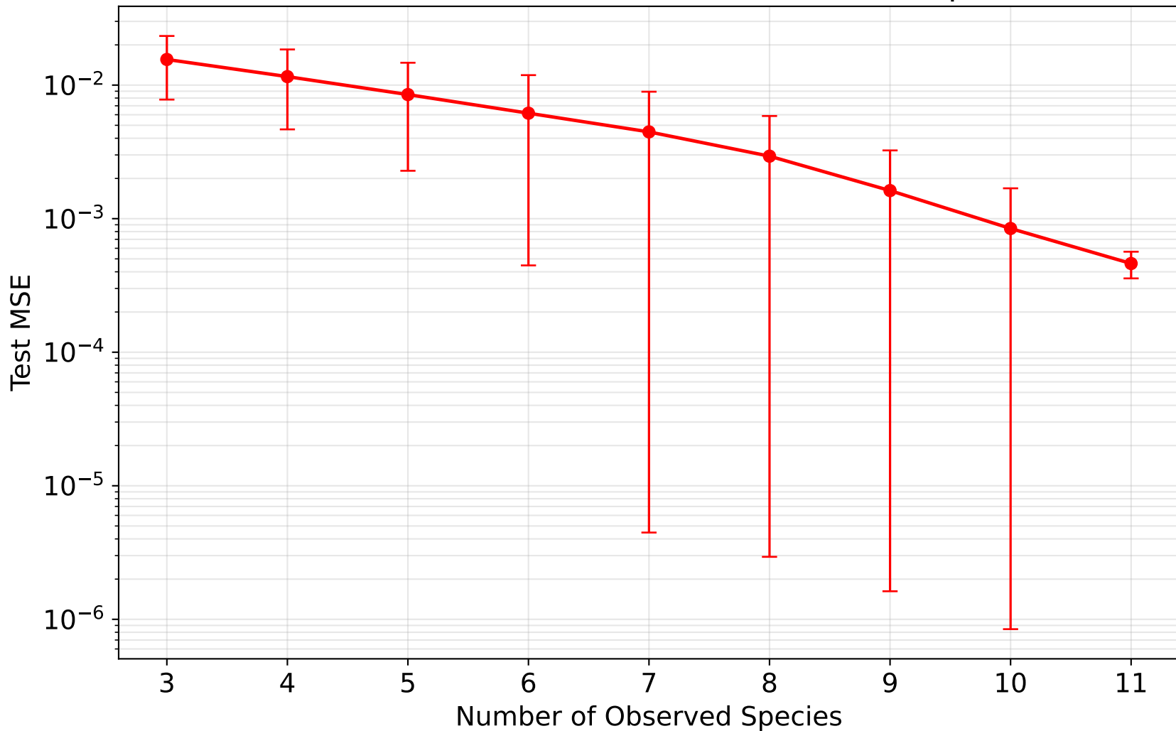
50, 50 — Test MSE vs number of observed species
